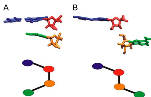
FIGURE 2 The pseudo-dihedral angle used to describe flipping of flanking bases A_{272} and A/G_{273} is defined by center of mass of the basepair C_{281}-G_{271} (blue), the G_{271} sugar (red), the sugar of flanking base for which \theta is calculated ( A_{272} or A/G_{273} ) (orange), and the base itself ( A_{272} or A/G_{273} ) (green). (A) Bulged-in and (B) bulged-out geometries of flanking bases.
